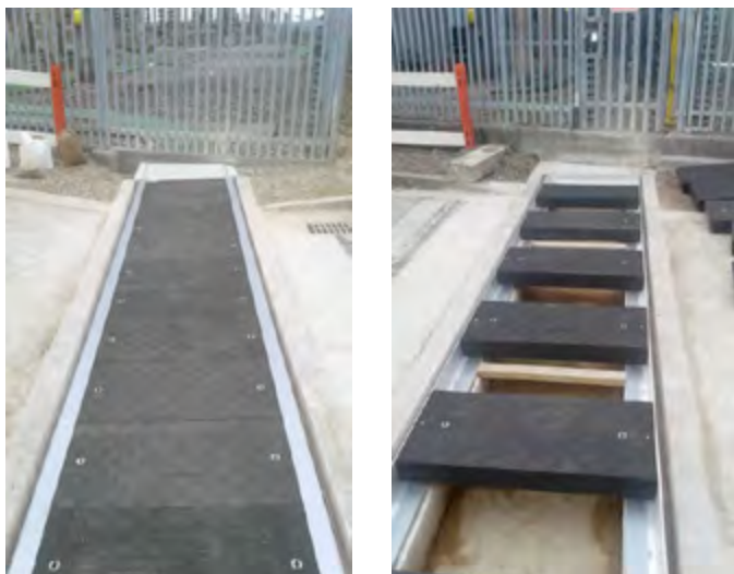
Fibrelite covers and frames were custom made to fit existing apertures, minimising installation time / upheaval to site
