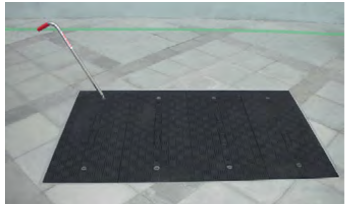
All Fibrelite trench covers can be safely manually lifted with the FL7 lifting handles (Image credit: Aguas de Cádiz)
