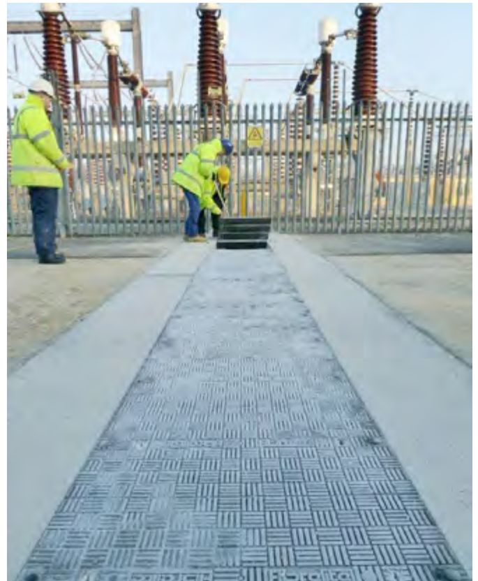
Fibrelite covers provide safe easy access to electrical cabling
